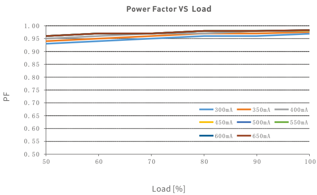
SE-20-300-650-G1T
