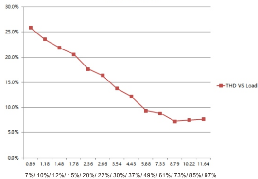
THD VS Load
