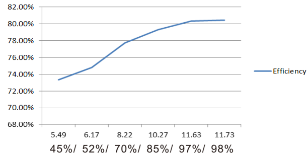
Typical Efficiency Vs Load
